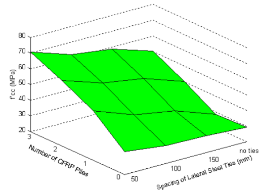
Figure 10. Sakai et al 2000 with addition of CFRP sheets as confinement ( D=200\text{mm} , d=185\text{mm} , L=600\text{mm} , p_{cc}=1.18\% , f_{ys}=376\text{Mpa} , and f'_c=29.8\text{ Mpa} )
