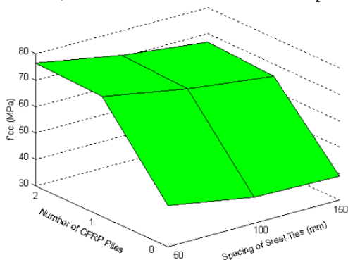
Figure 8. Mander et al 1988b with addition of CFRP sheets as confinement ( D=500\text{mm} , d=438\text{mm} , L=1500\text{mm} , p_{cc}=1.6\% , f_{ys}=340\text{Mpa} , lateral steel bar diameter= 12\text{mm} , and f'_c=28\text{ Mpa} )
