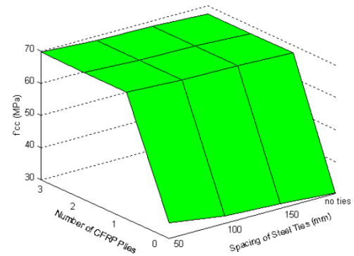
Figure 9. Hoshikuma 1997 with addition of CFRP sheets as confinement ( D=500\text{mm} , d=500\text{mm} , L=1500\text{mm} , p_{cc}=1.01\% , f_{ys}=295\text{Mpa} , and f'_c=28.8\text{ Mpa} )
