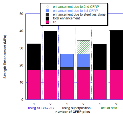
Figure 11. Strength Enhancement using Li and Fang 2004 Data ( D=300\text{mm} , d=250\text{mm} , L=600\text{mm} , \rho_s = 1.41\% , \rho_{cc}=0.76\% , f_{yh}=274.7\text{Mpa} , t=0.11\text{mm} , f_{yfrp}=4120.2\text{Mpa} , f_c'=17.2\text{Mpa} )
