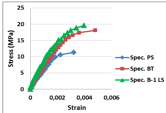
Figure 14. Stress strain curve of specimens
